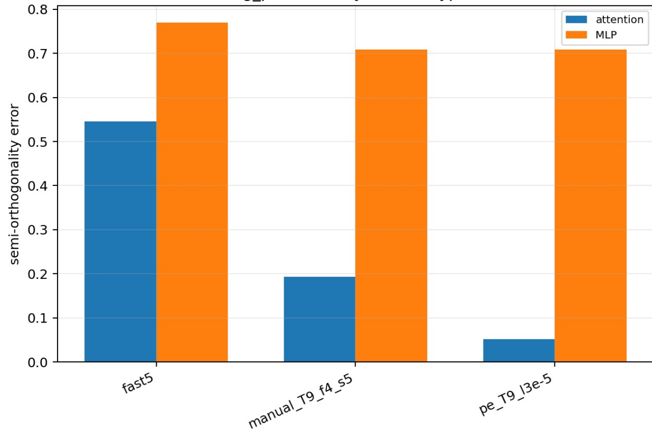
g_post error by module type
