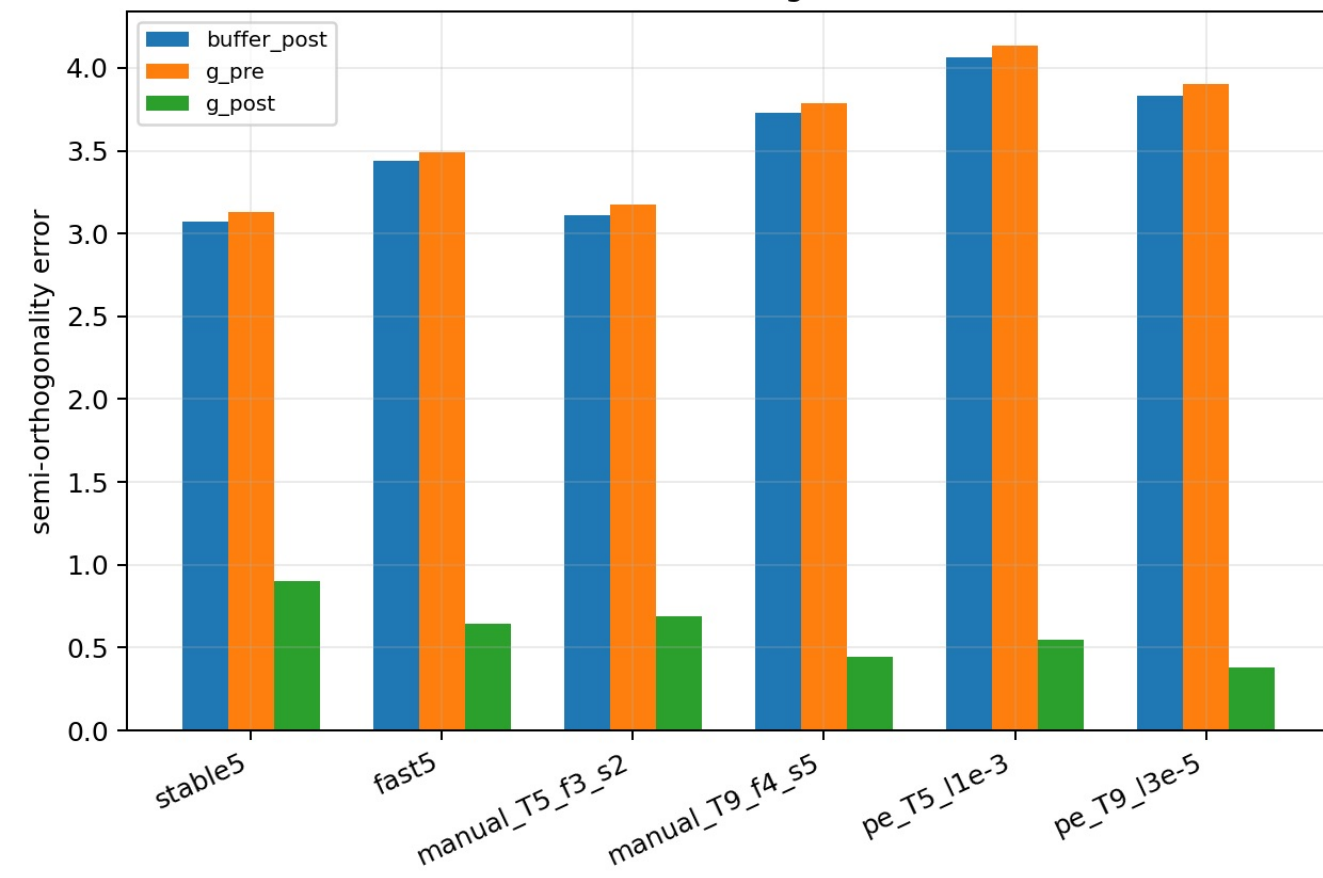
Before / after orthogonalization
