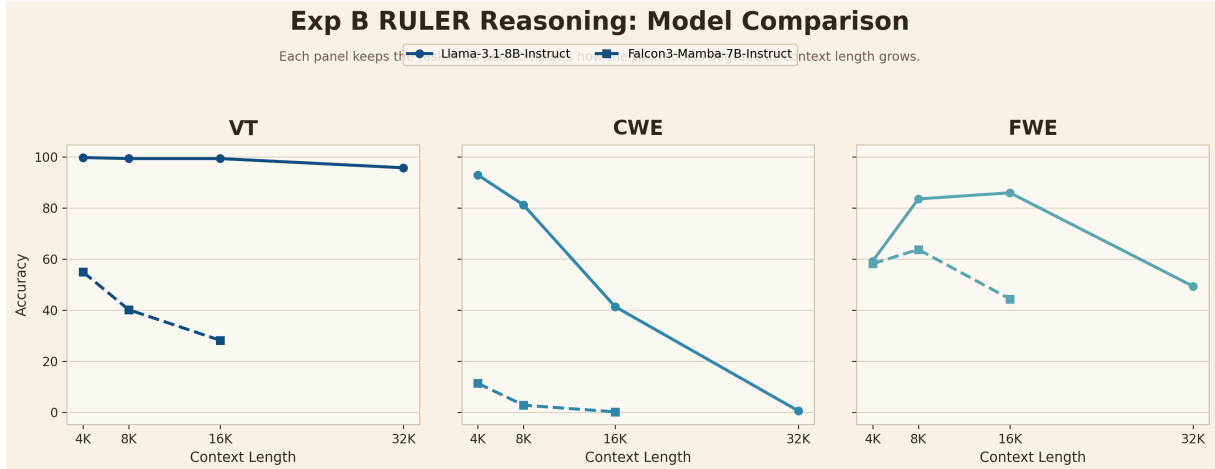
Figure 2: Exp B RULER reasoning comparison curves. Each panel fixes one task and compares how Llama-3.1-8B-Instruct and Falcon3-Mamba-7B-Instruct degrade as context length grows.
