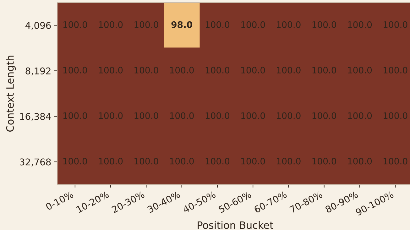
NIAH Single-Key Heatmap
