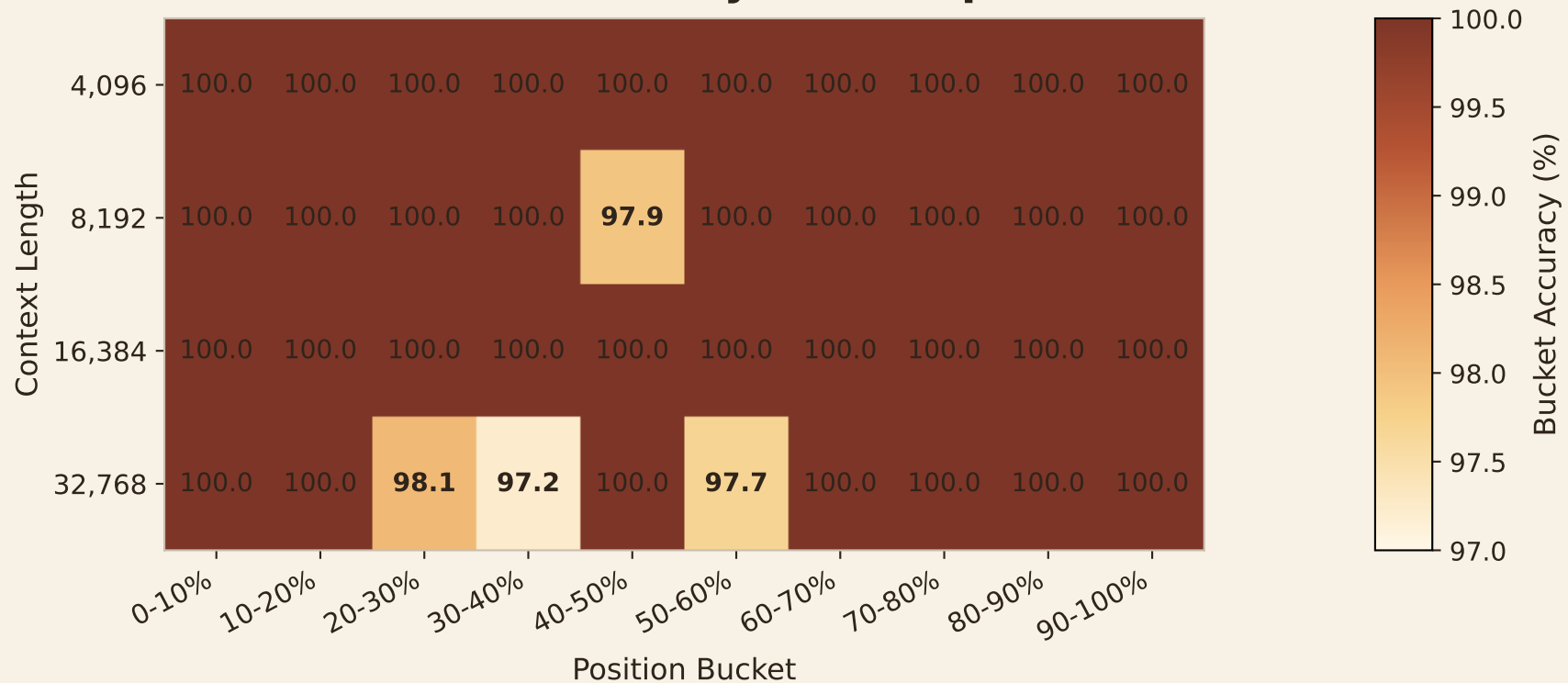
NIAH Multi-Key Heatmap
