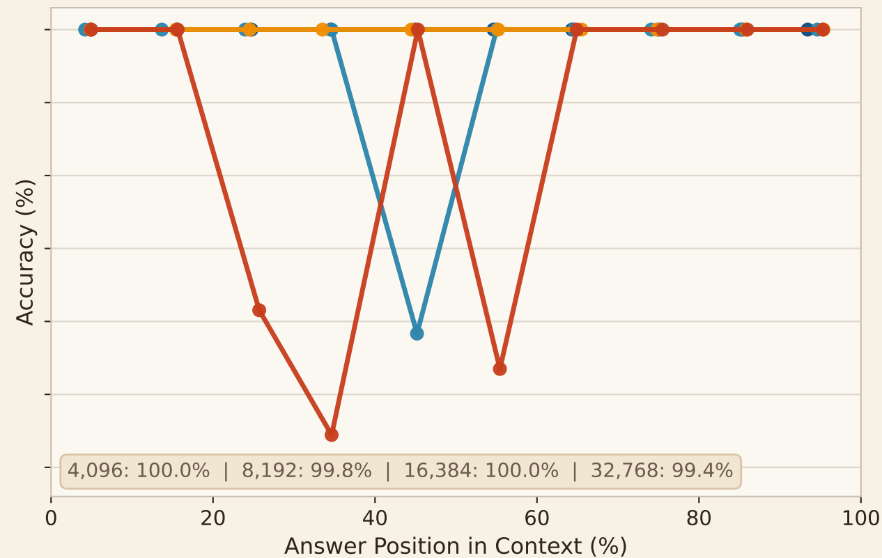
NIAH Multi-Key
