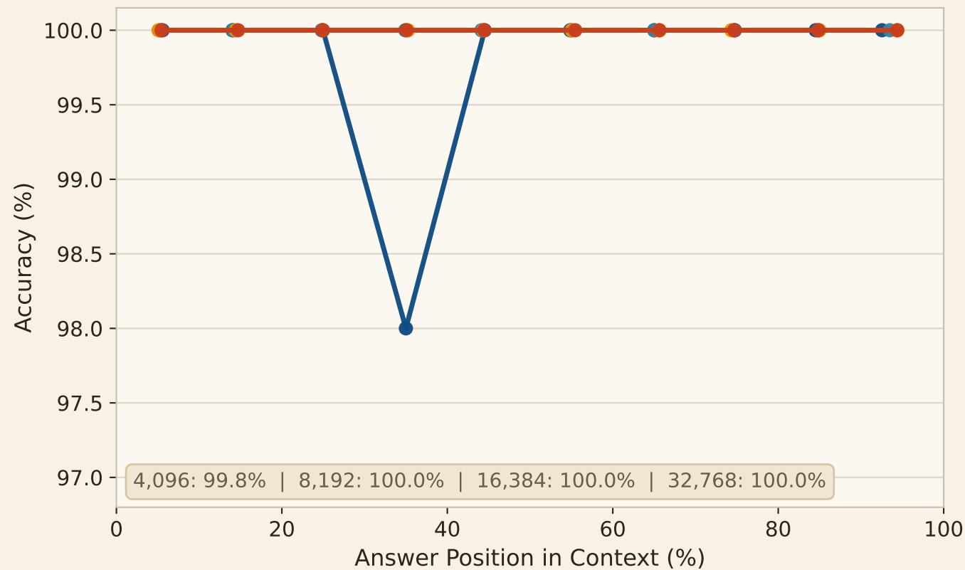
NIAH Single-Key
