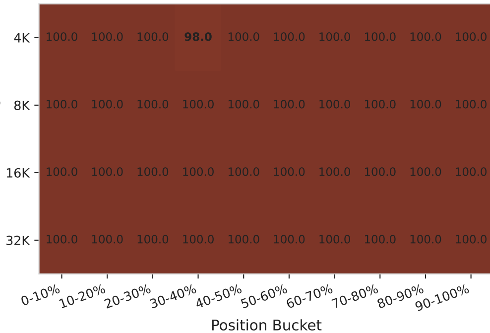
Llama-3.1-8B-Instruct
