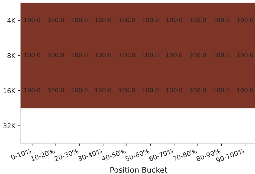
Falcon3-Mamba-7B-Instruct
