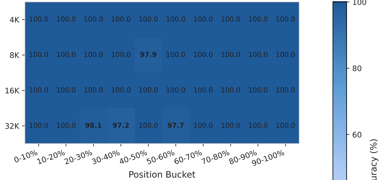
NIAH Multi-Key
