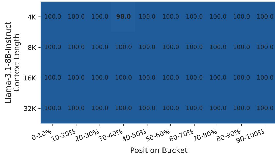
NIAH Single-Key
