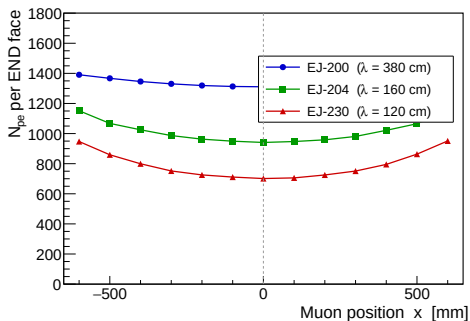
N_{pe}/end vs x for three scintillators. EJ-200 highest, EJ-230 lowest but fastest decay.
