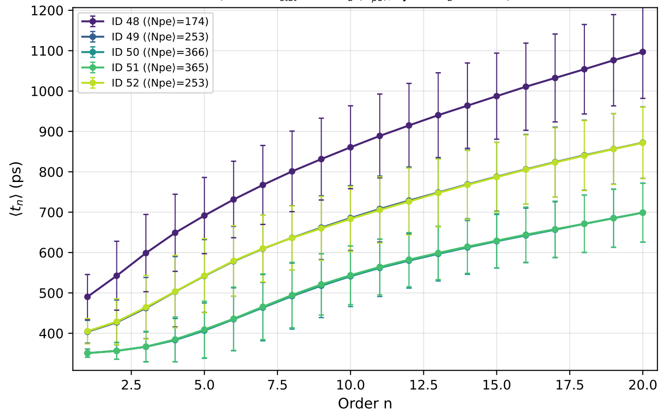
F2 — EJ-230 Run 4: x=+0 mm, nearest \pm 2 cluster (dotted: \sigma_{stat} = \sqrt{n} \cdot \tau_d / \langle N_{pe} \rangle , EJ-230 \tau_d = 1.5 ns)
