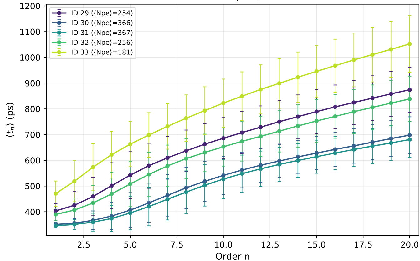
F2 — EJ-230 Run 3: x=-400 mm, nearest \pm 2 cluster (dotted: \sigma_{stat} = \sqrt{n} \cdot \tau_d / \langle N_{pe} \rangle , EJ-230 \tau_d = 1.5 ns)
