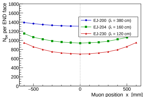
N_{\text{pe}}/\text{end} vs x for three scintillators. EJ-200 highest, EJ-230 lowest but fastest decay.
