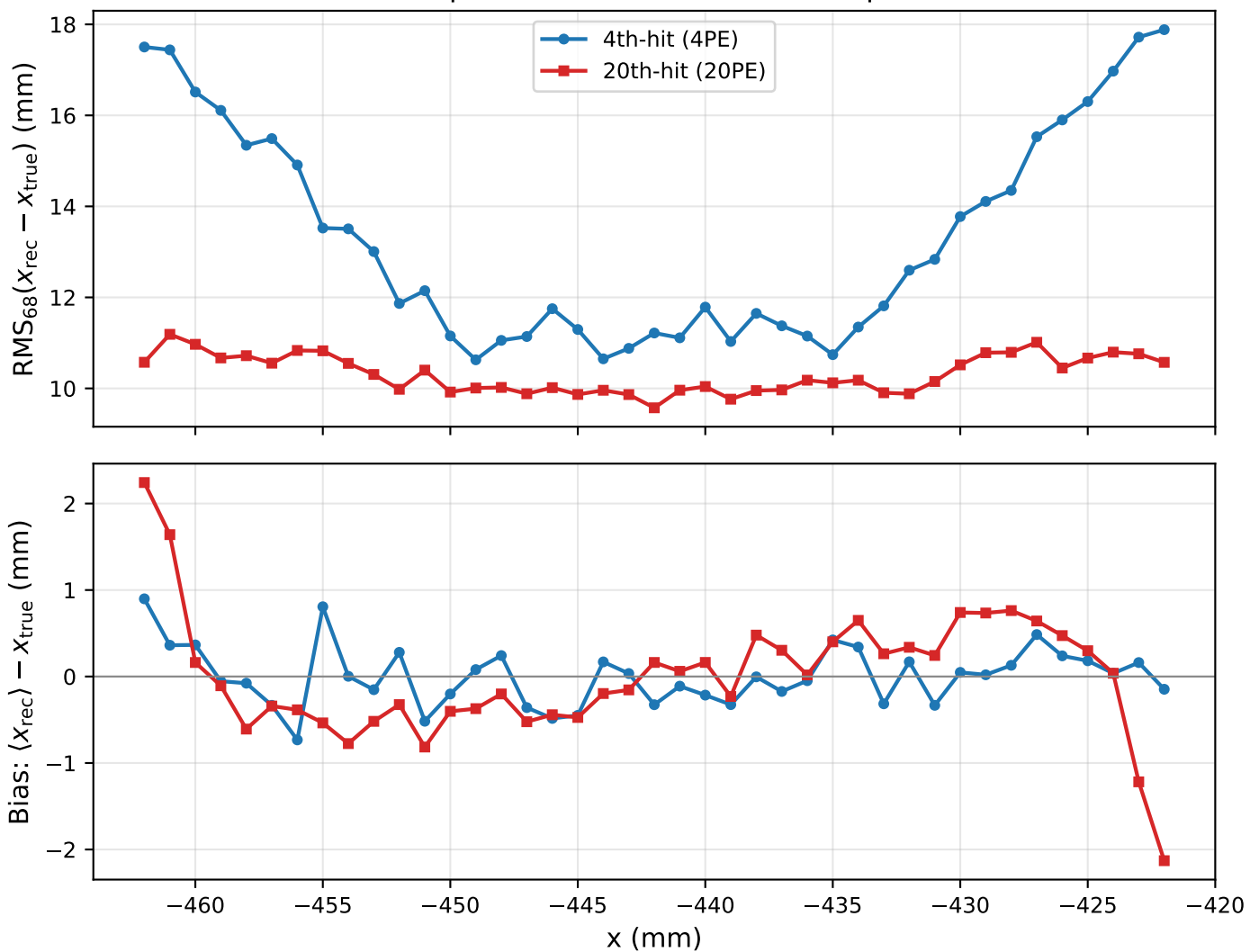
LOO-CV position resolution vs. beam position
