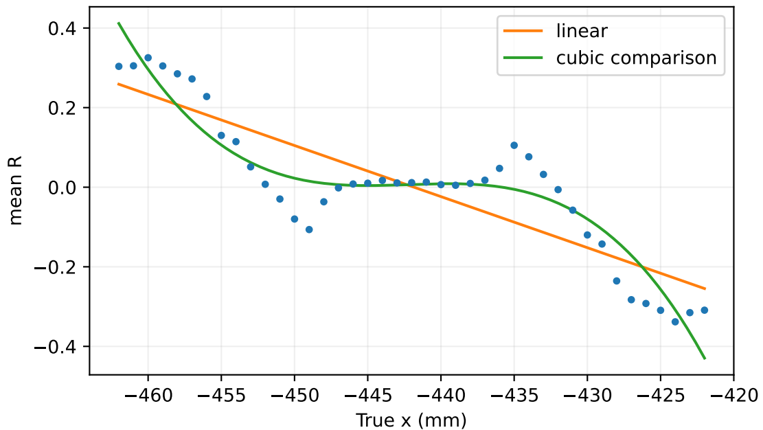
Ratio calibration; linear chi2/ndf=3969.57
