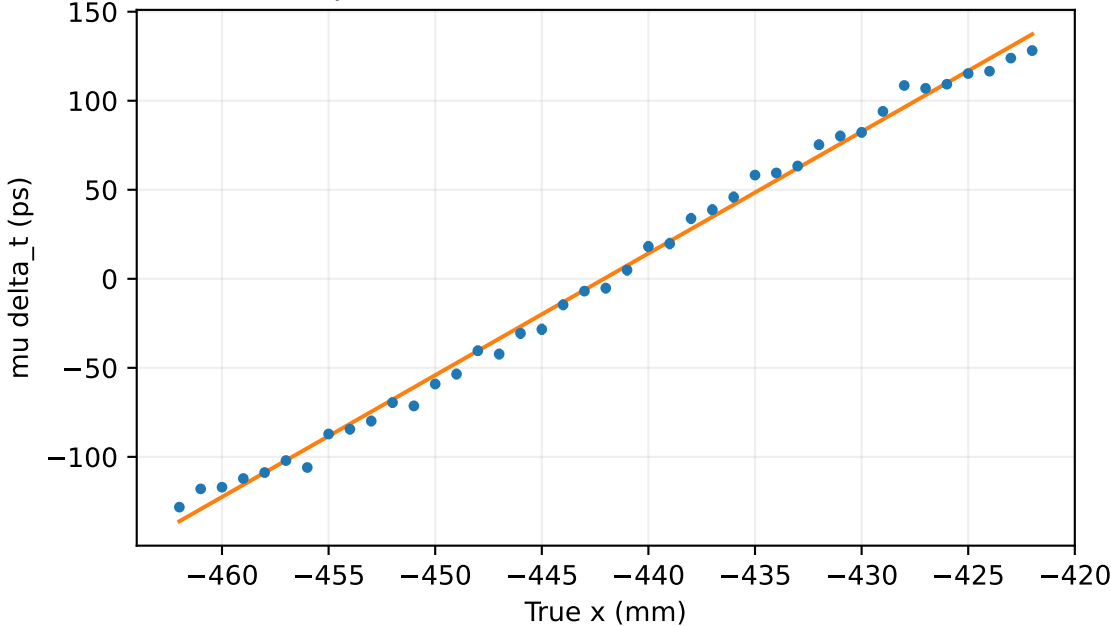
Temporal linear calibration; chi2/ndf=4.70
