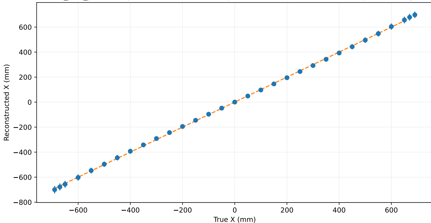
dt_end_pool LOO prediction — simulation prediction — EJ-204 — intrinsic optical timing
