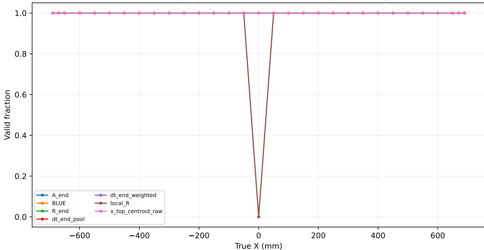
simulation prediction — Ej-204 — intrinsic optical timing
