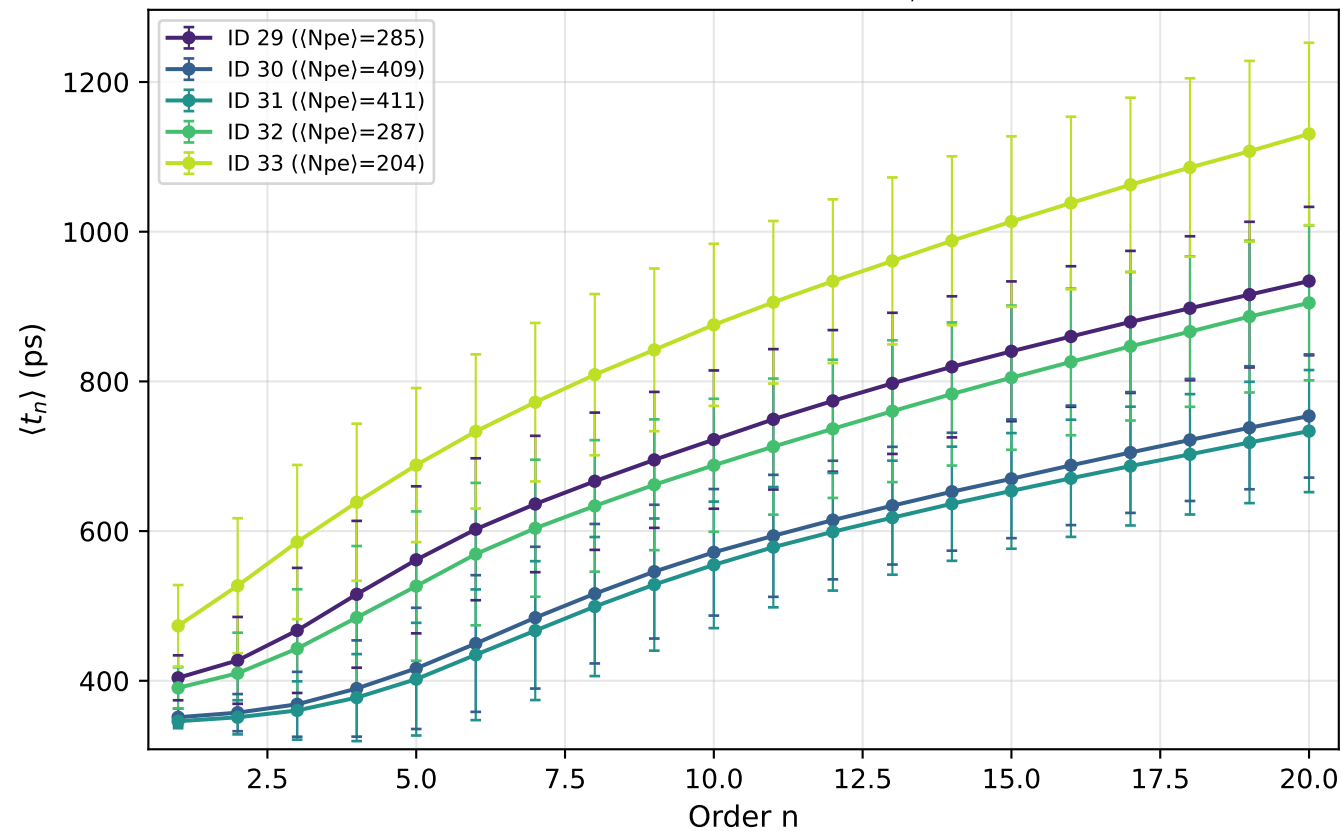
F2 — Run 3: x=-400 mm, nearest \pm 2 cluster (dashed: stat floor \sqrt{n} \cdot \tau_d / \langle N_{pe} \rangle )
