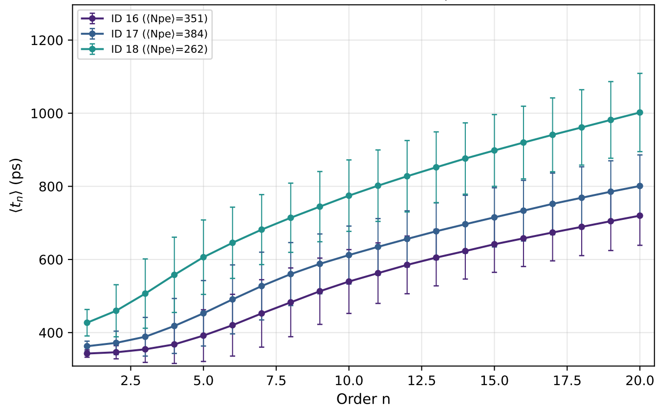
F2 — Run 1: x=-690 mm, nearest \pm 2 cluster (dashed: stat floor \sqrt{n} \cdot \tau_d / \langle N_{pe} \rangle )
