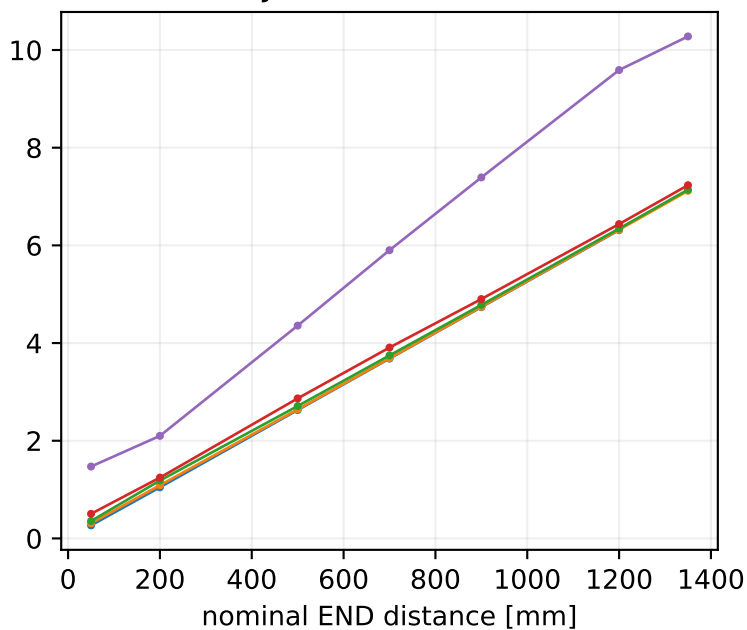
EJ-204, Cherenkov
