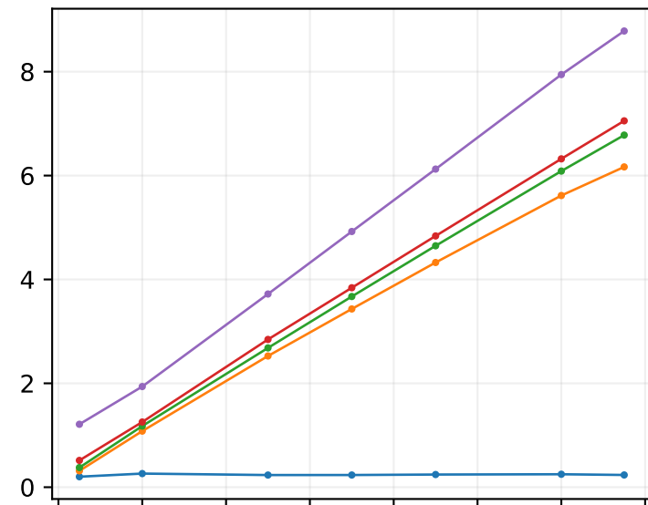
EJ-230, scintillation
