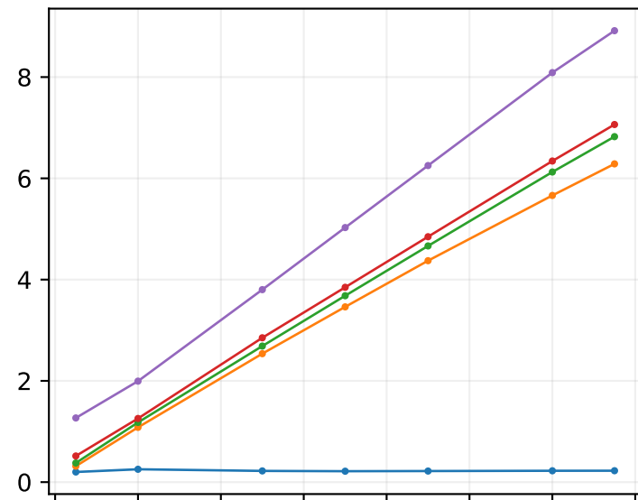
EJ-204, scintillation
