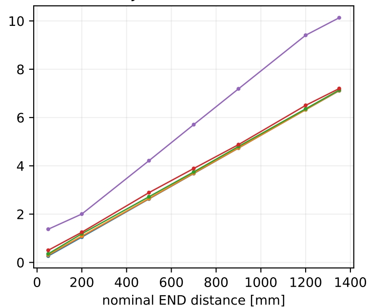
EJ-230, Cherenkov
