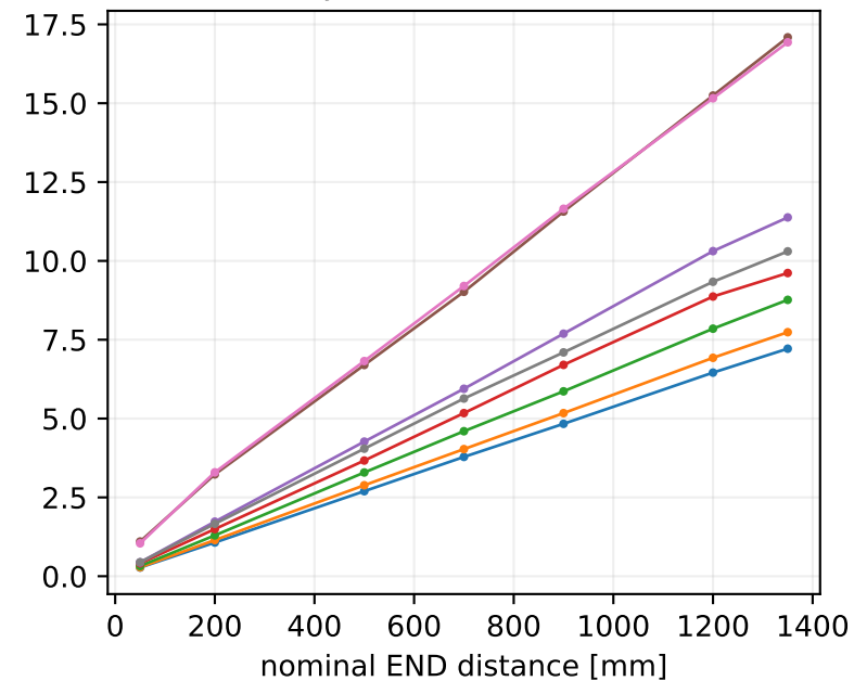
EJ-230, Cherenkov
