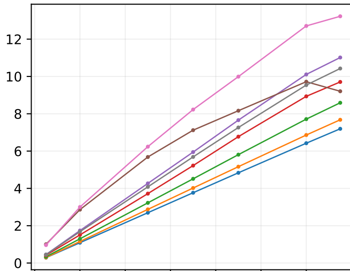
EJ-204, scintillation
