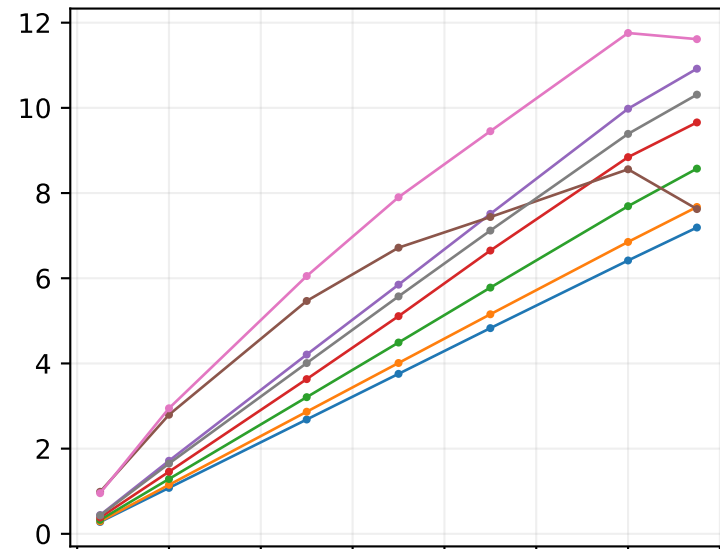
EJ-230, scintillation
