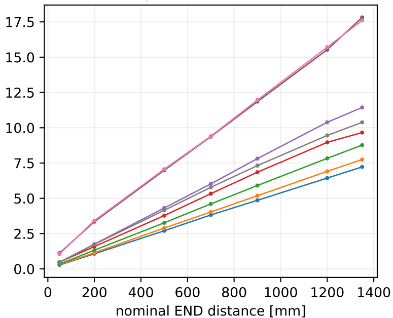
EJ-204, Cherenkov
