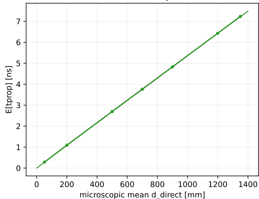
scintillation, first by source
