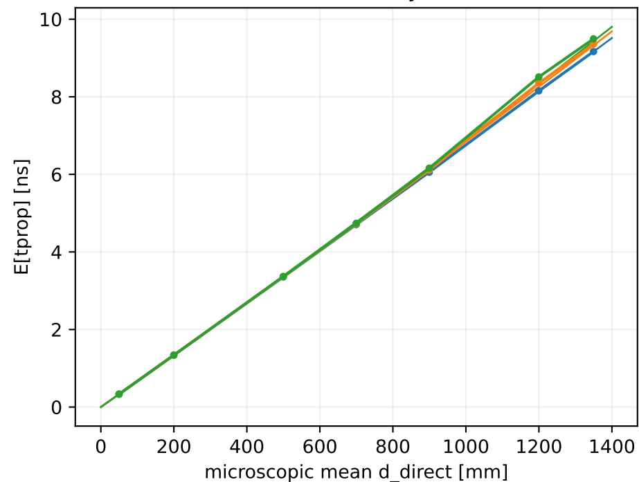
Cherenkov, first by source
