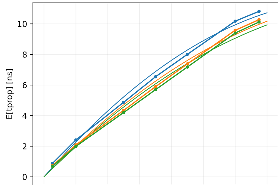
Cherenkov, all photons
