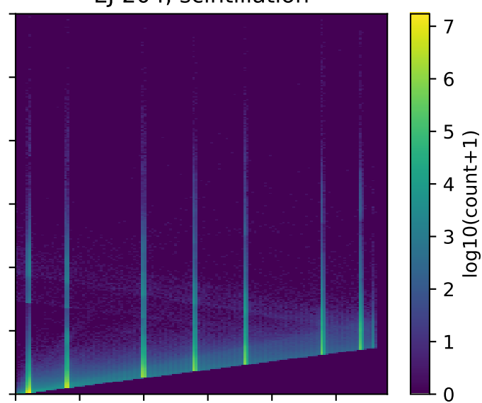
EJ-204, scintillation
