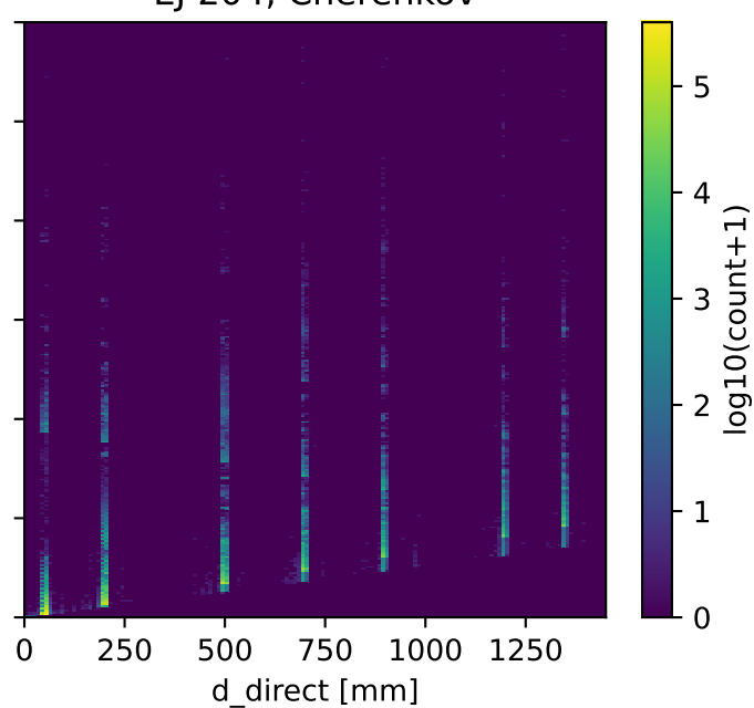
EJ-204, Cherenkov
