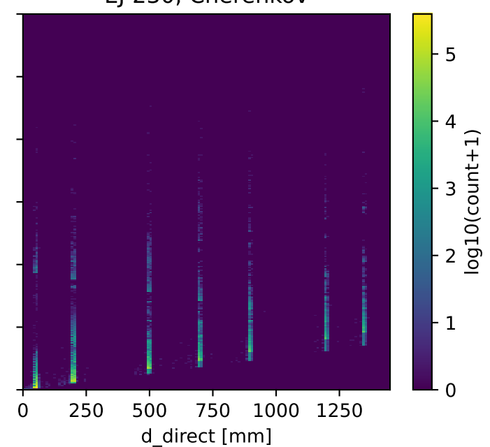
EJ-230, Cherenkov
