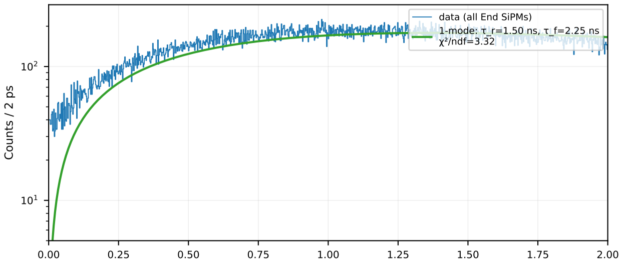
EJ-204 x = +0 mm — window 0-2 ns (2 ps bin, log-Y)
