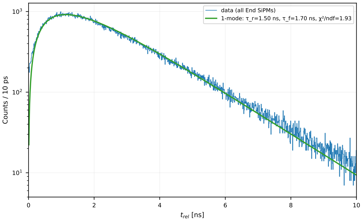
EJ-204 x = +0 mm — window 0-10 ns (10 ps bin, log-Y)
