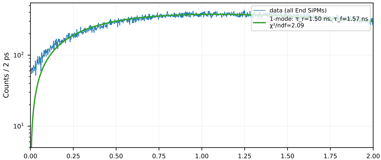
EJ-204 x = +400 mm — window 0-2 ns (2 ps bin, log-Y)
