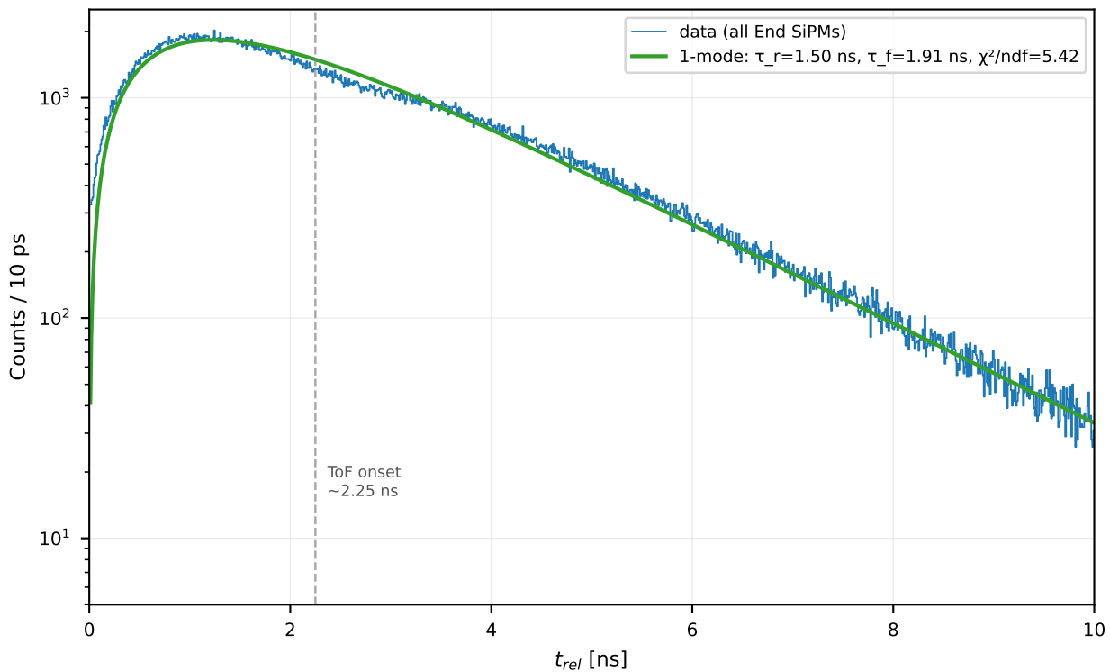
EJ-204 x = +400 mm — window 0-10 ns (10 ps bin, log-Y)
