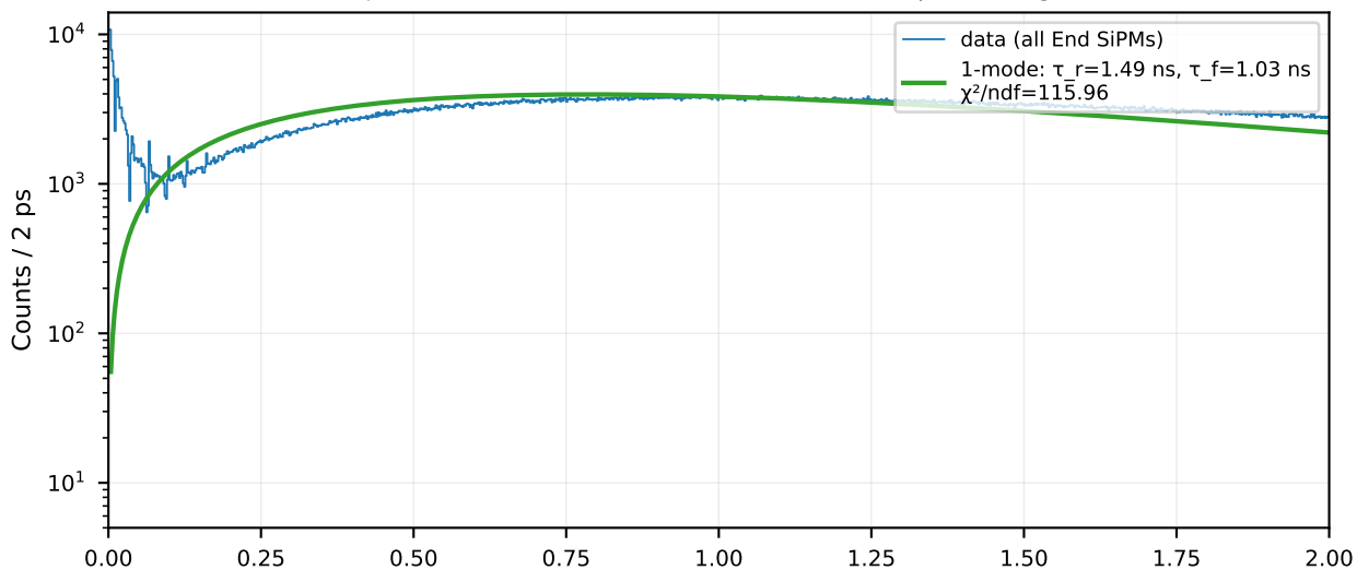
EJ-204 x = +690 mm — window 0-2 ns (2 ps bin, log-Y)
