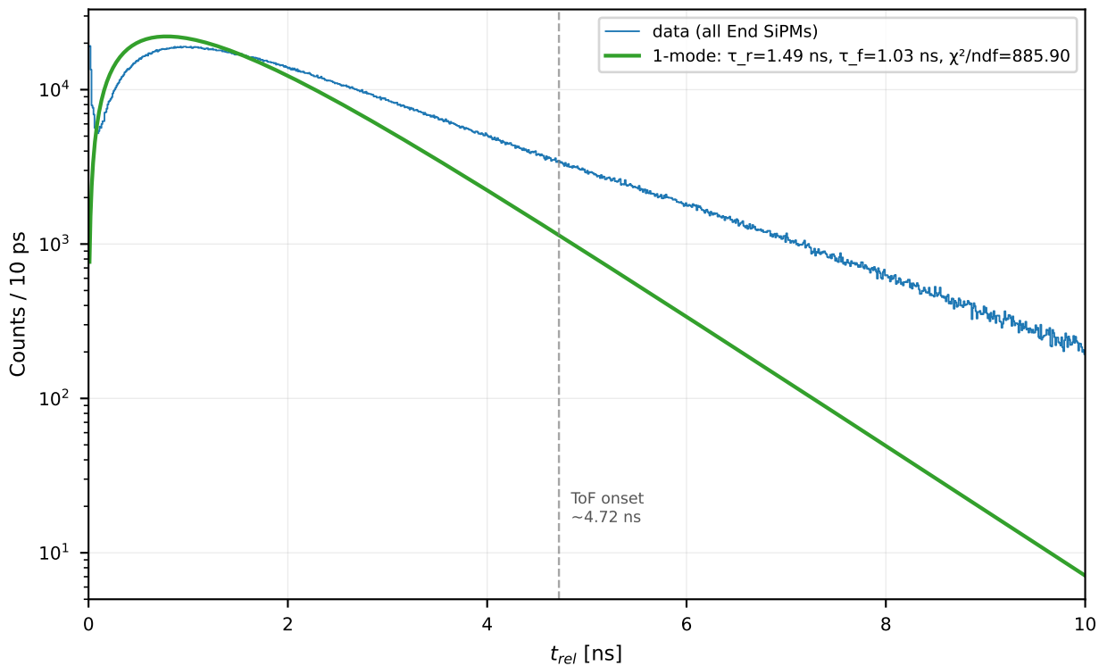
EJ-204 x = +690 mm — window 0-10 ns (10 ps bin, log-Y)
