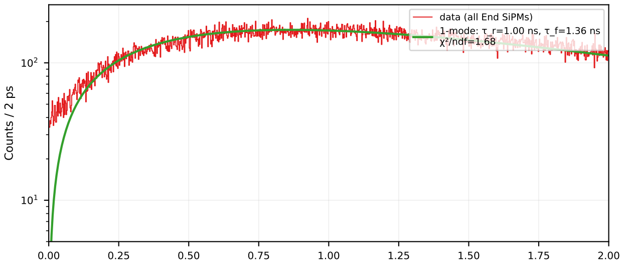
EJ-230 x = +0 mm — window 0-2 ns (2 ps bin, log-Y)
