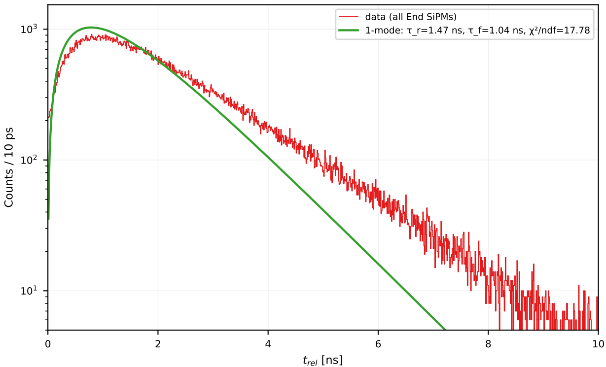
EJ-230 x = +0 mm — window 0-10 ns (10 ps bin, log-Y)
