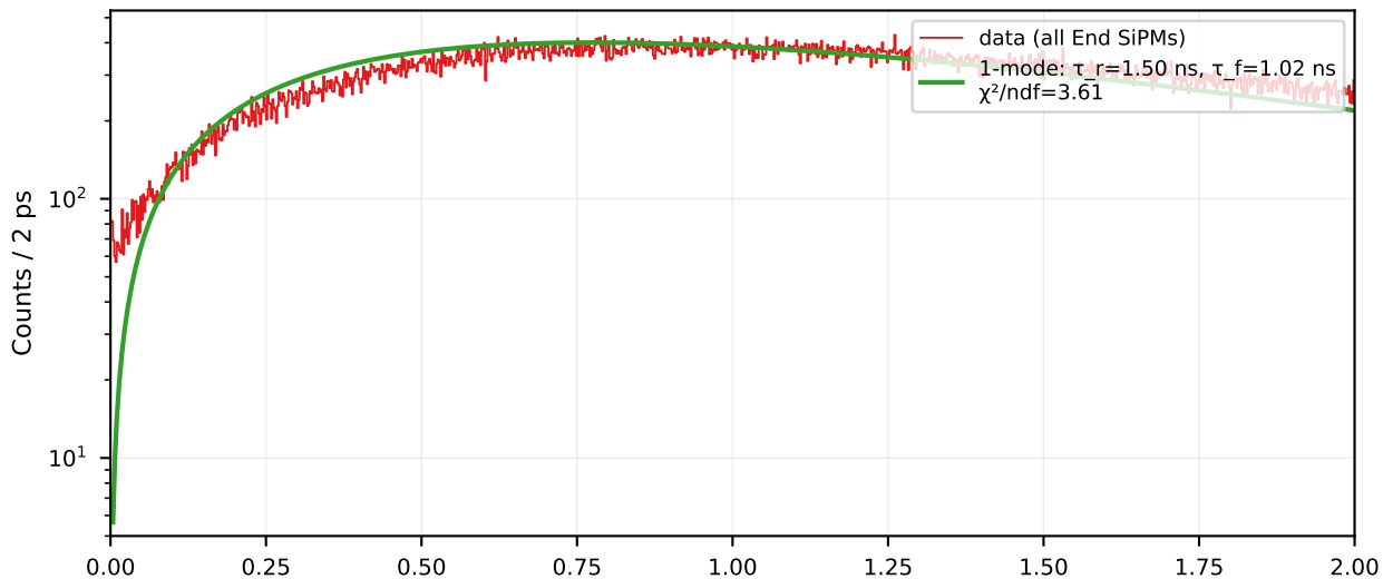
EJ-230 x = +400 mm — window 0-2 ns (2 ps bin, log-Y)
