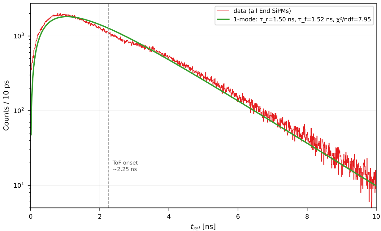
EJ-230 x = +400 mm — window 0-10 ns (10 ps bin, log-Y)
