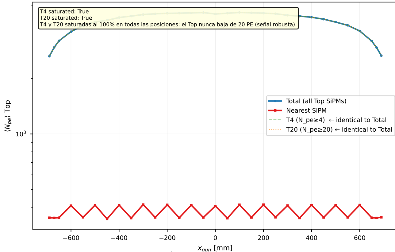
F4 — N_{pe} Top profiles vs position (EndTop EJ-204, log-Y)
