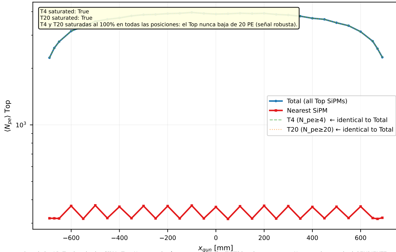
F4 — N_{pe} Top profiles vs position (EndTop EJ-230, log-Y)
