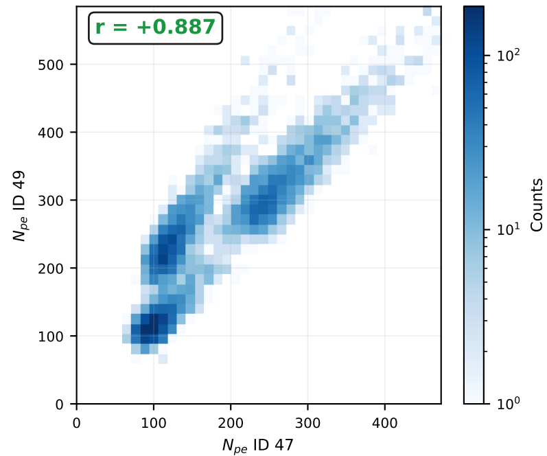
Pair C: IDs 47/49 (X=-72mm / -32mm, sep 40mm; control) (sep=40 mm)
