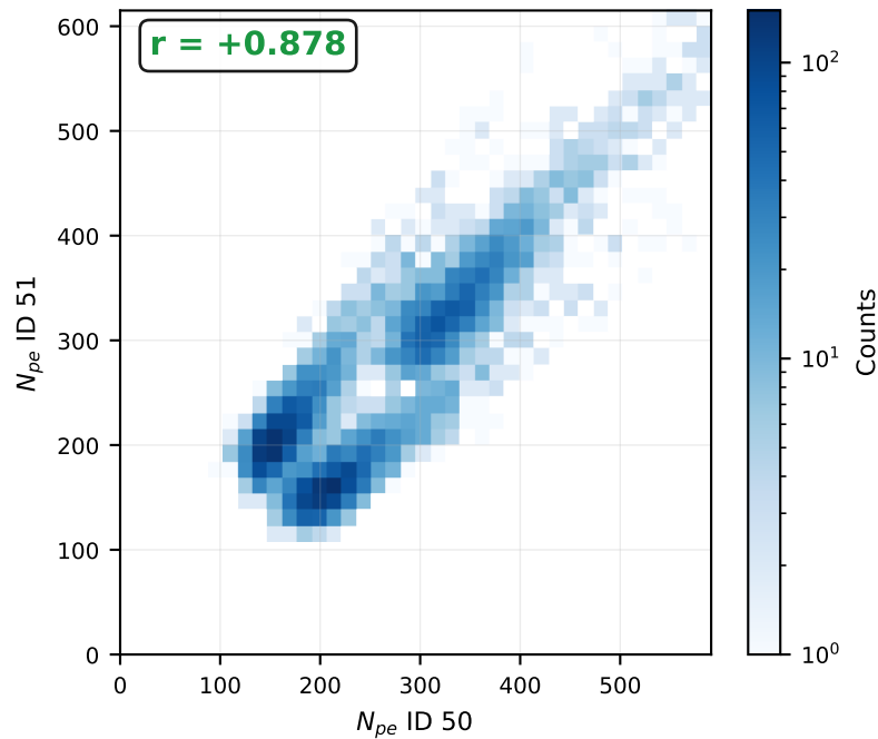
Pair B: IDs 50/51 (X=-12mm / +12mm, sep 24mm, adjacent gap) (sep=24 mm)
