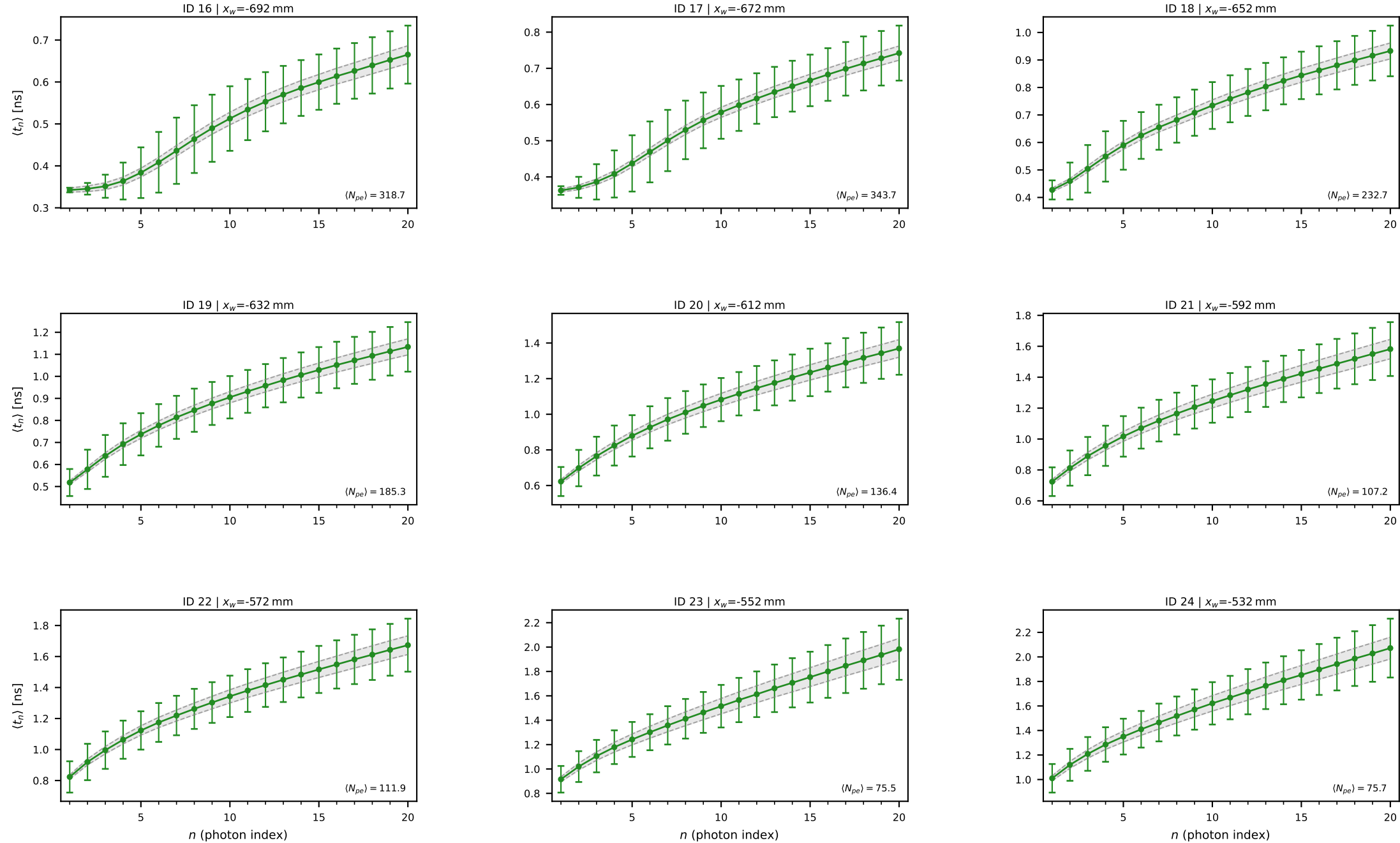
F7 — Order-statistic arrival time ( t_n ) per Top channel | x_{\text{gun}} = -690 mm (EJ-230 EndTop) Error bars = RMS (event-to-event). Dashed band: stat.\ floor \sqrt{n} \tau_d / \langle N_{pe} \rangle , \tau_d = 1.5 ns
