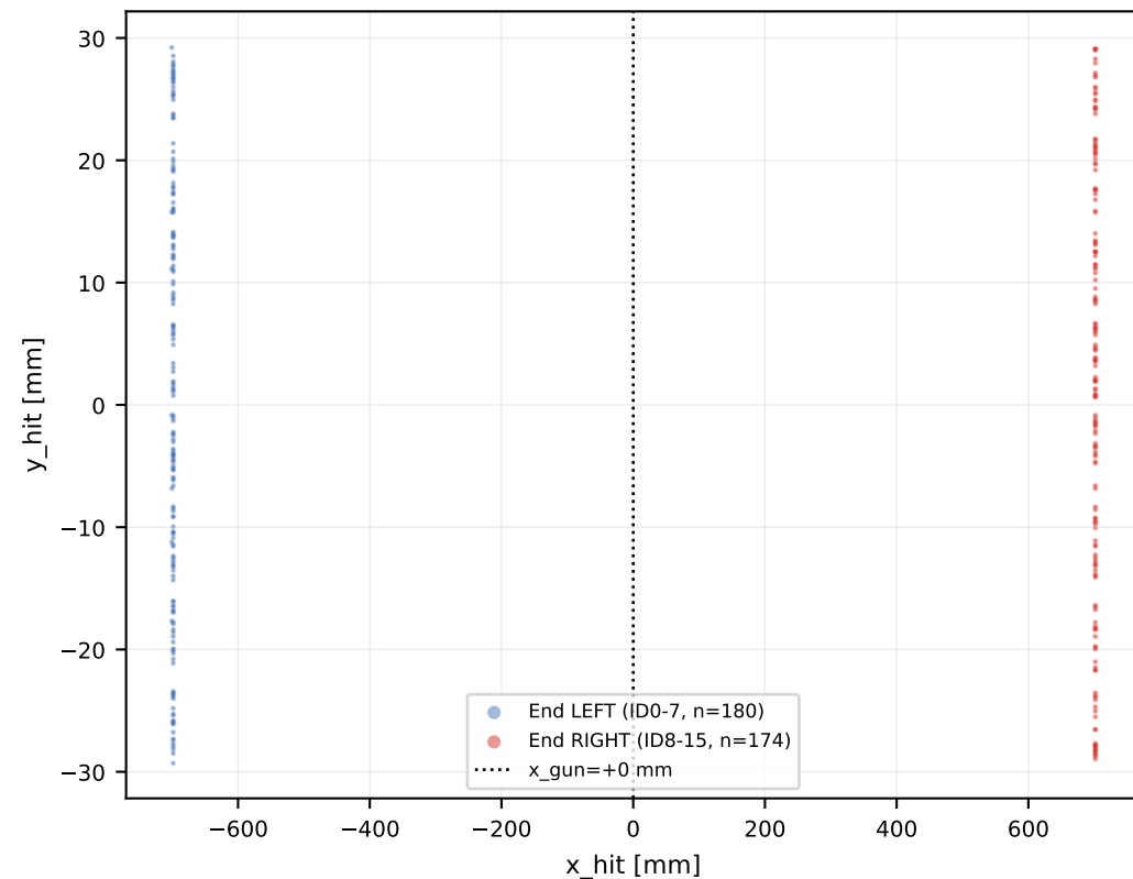
Longitudinal view (x vs y) EJ-230 x gun =+0 mm ev=1546
