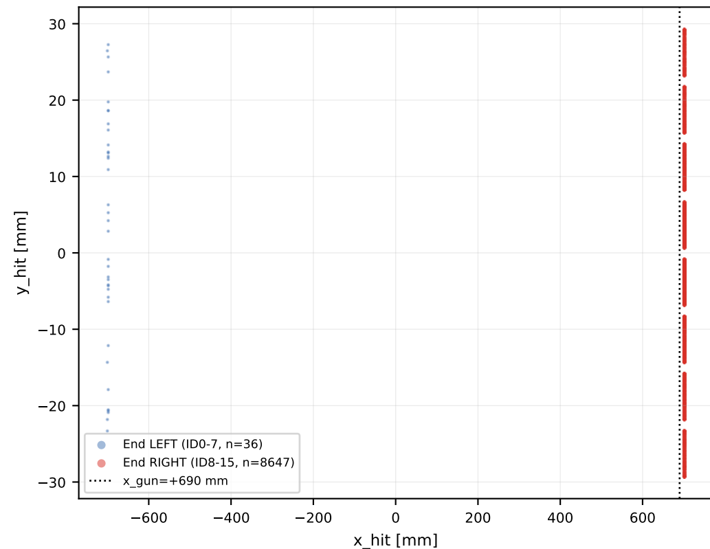
Longitudinal view (x vs y) EJ-230 x_gun=+690 mm ev=552
