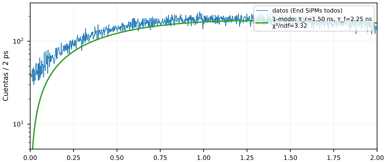
EJ-204 x = +0 mm — ventana 0-2 ns (bin 2 ps, log-Y)
