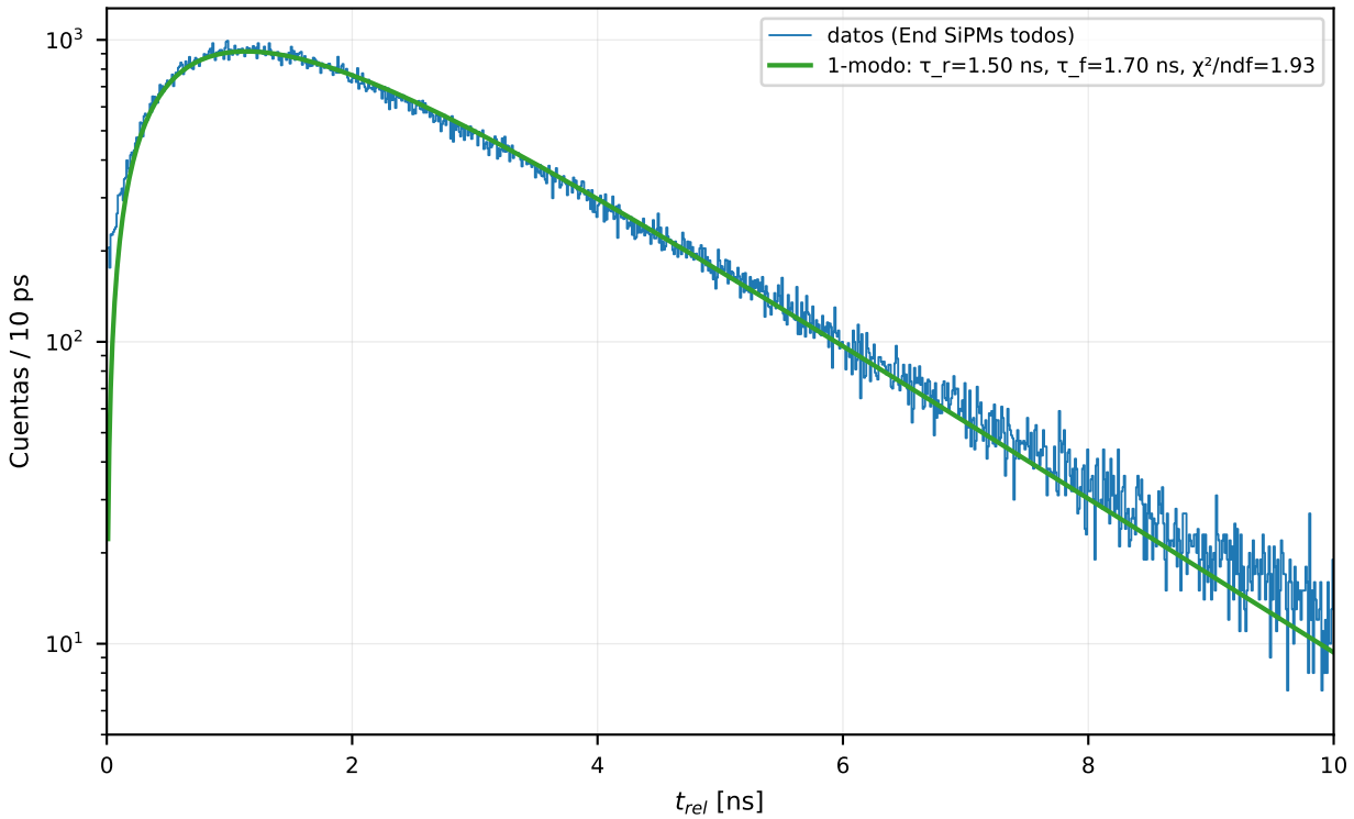
EJ-204 x = +0 mm — ventana 0-10 ns (bin 10 ps, log-Y)
