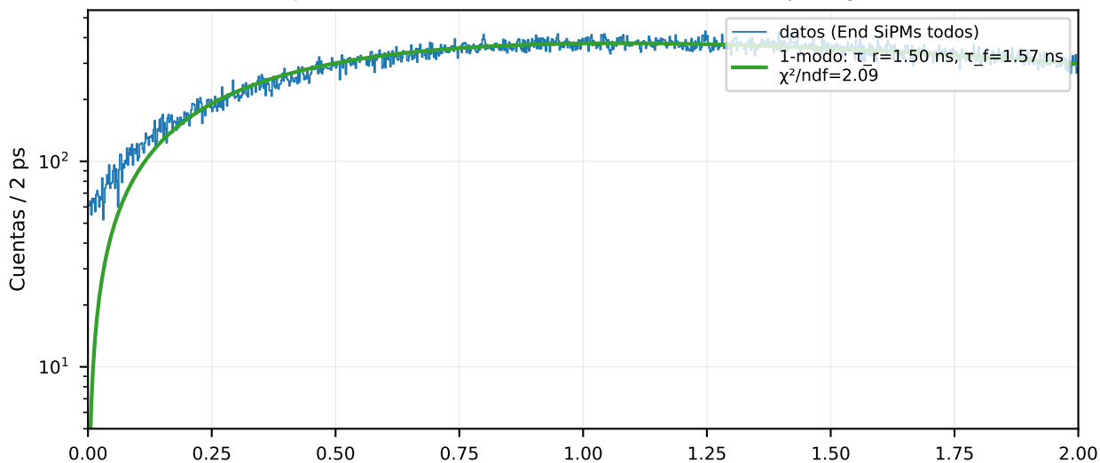
EJ-204 x = +400 mm — ventana 0-2 ns (bin 2 ps, log-Y)
