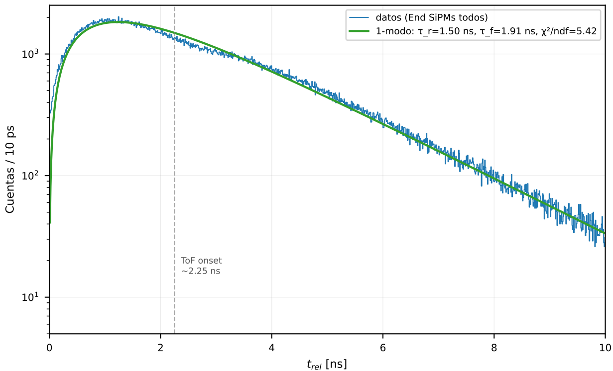
EJ-204 x = +400 mm — ventana 0-10 ns (bin 10 ps, log-Y)
