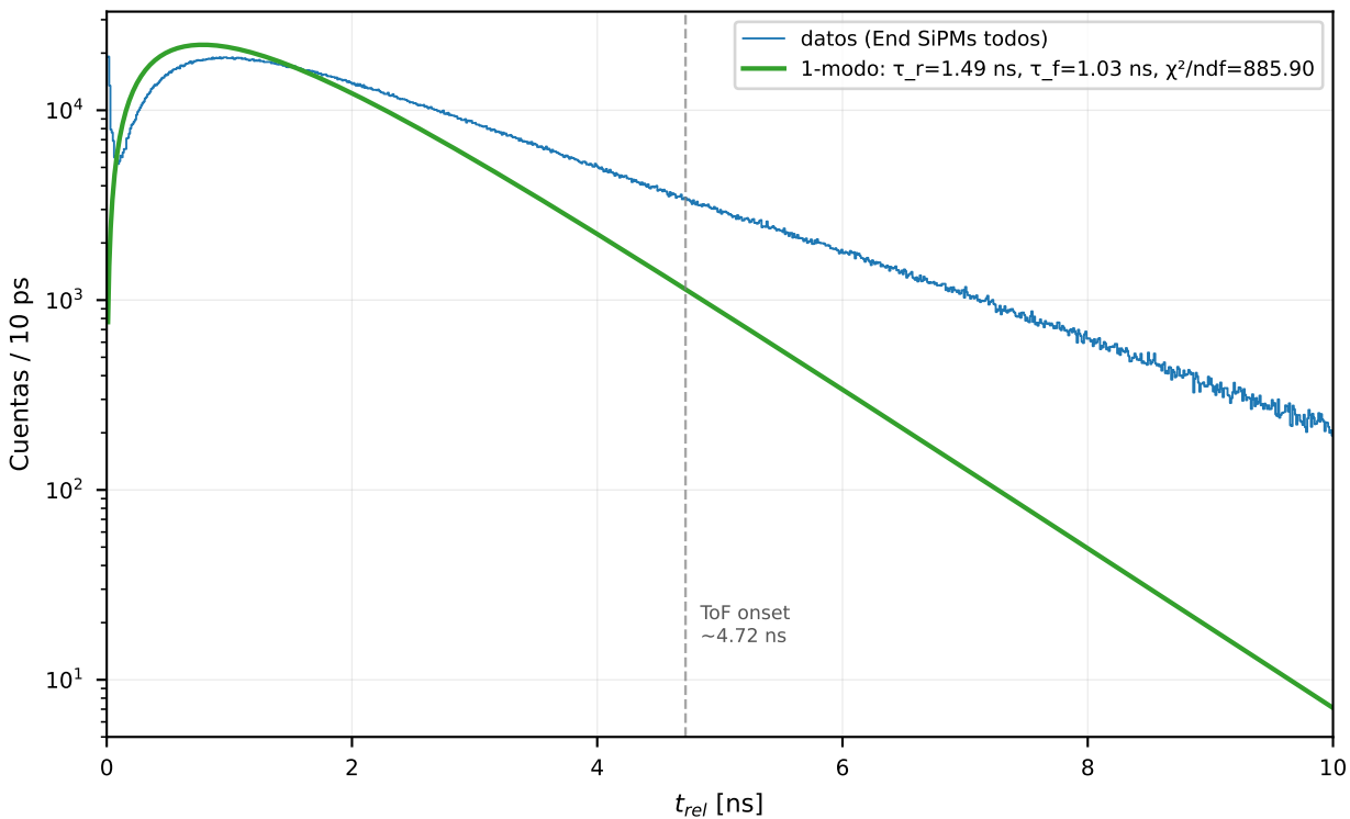
EJ-204 x = +690 mm — ventana 0-10 ns (bin 10 ps, log-Y)
