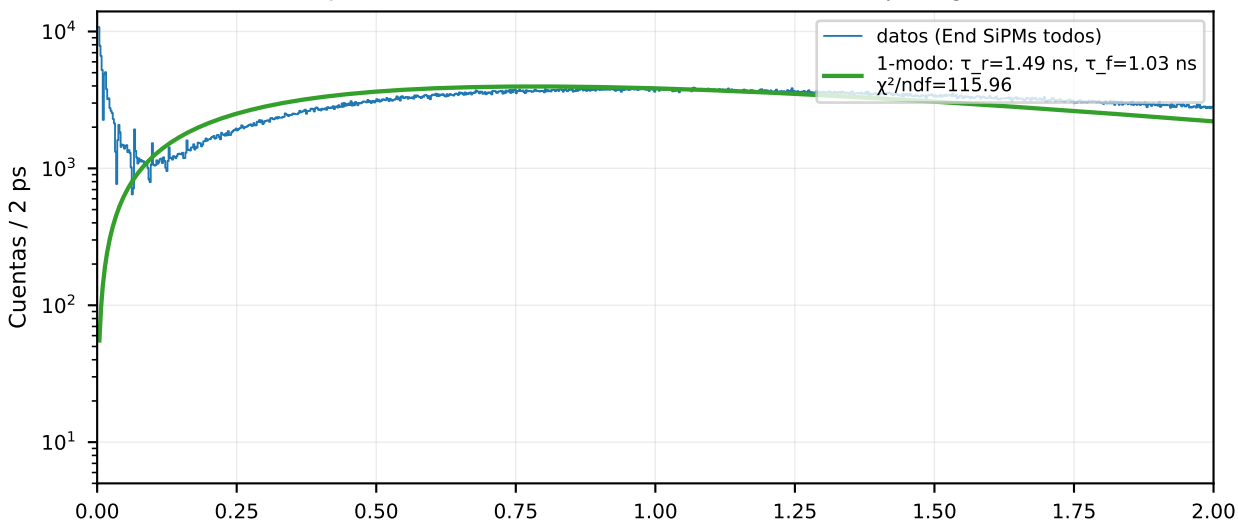
EJ-204 x = +690 mm — ventana 0-2 ns (bin 2 ps, log-Y)
