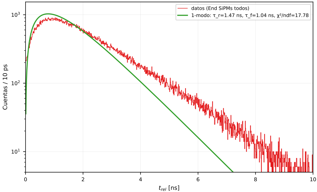
EJ-230 x = +0 mm — ventana 0-10 ns (bin 10 ps, log-Y)
