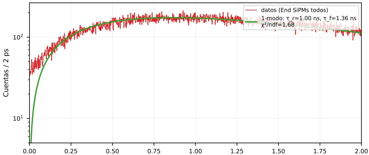
EJ-230 x = +0 mm — ventana 0-2 ns (bin 2 ps, log-Y)
