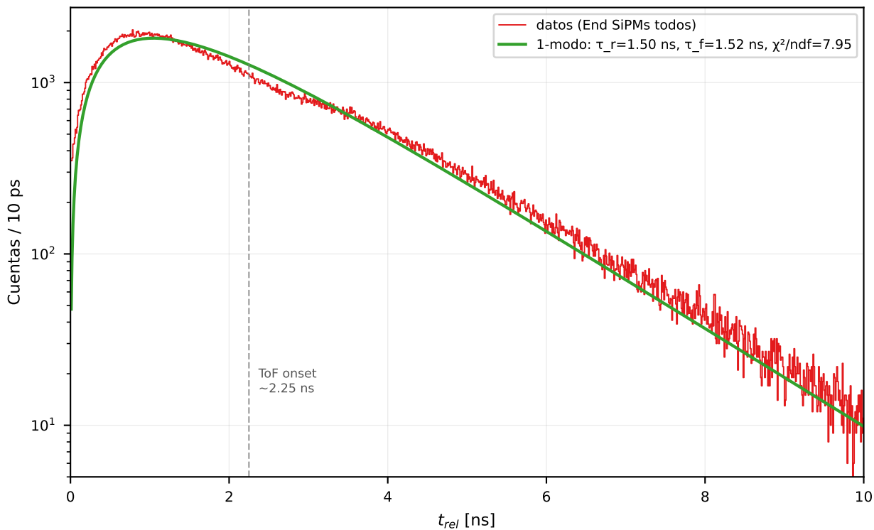
EJ-230 x = +400 mm — ventana 0-10 ns (bin 10 ps, log-Y)
