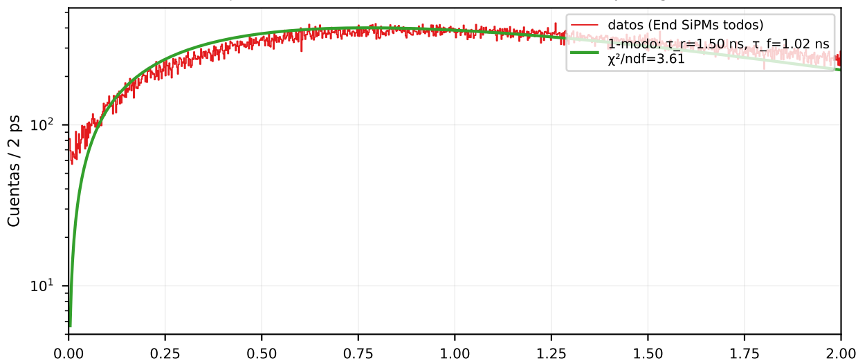
EJ-230 x = +400 mm — ventana 0-2 ns (bin 2 ps, log-Y)
