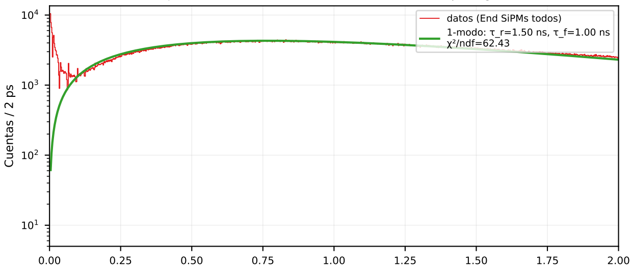
EJ-230 x = +690 mm — ventana 0-2 ns (bin 2 ps, log-Y)
