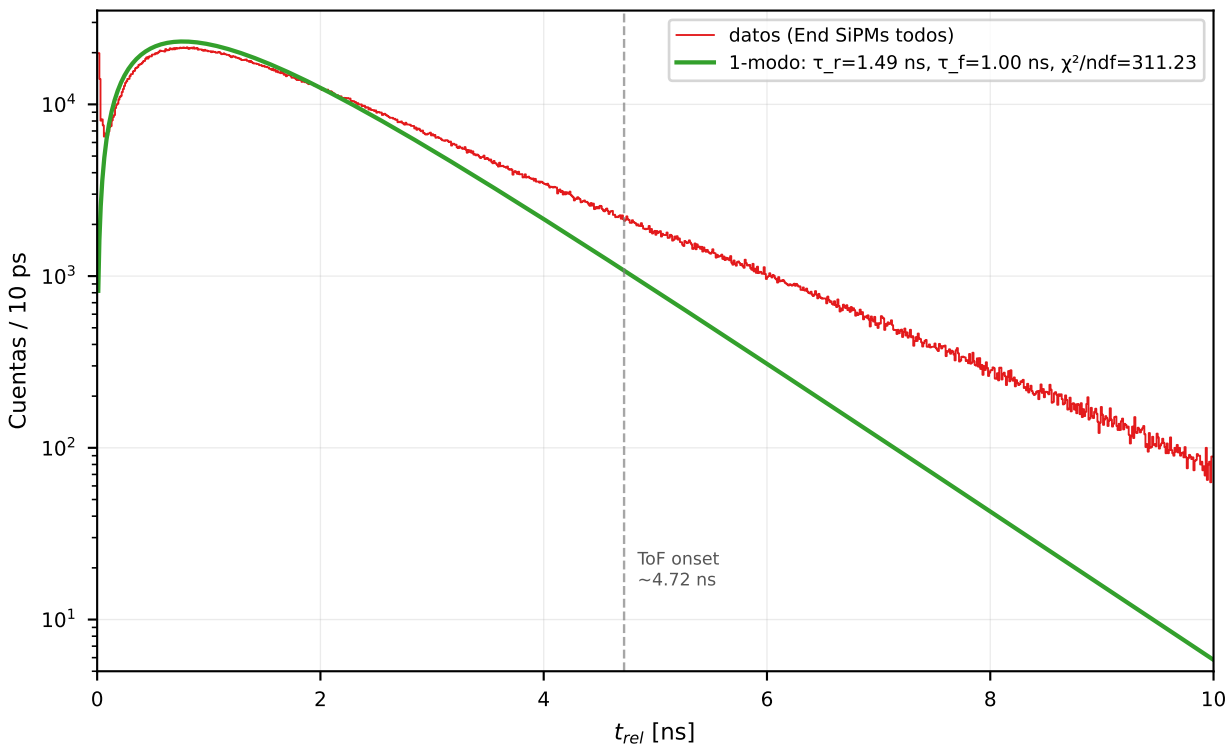
EJ-230 x = +690 mm — ventana 0-10 ns (bin 10 ps, log-Y)
