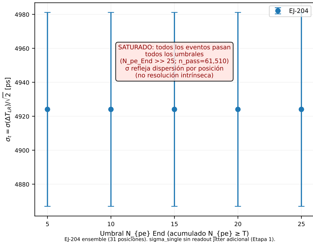
F2 — Ensemble \sigma_t vs umbral N_{\{pe\}} (EJ-204)
