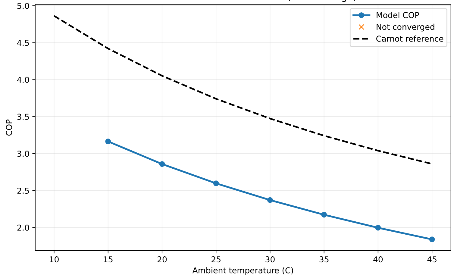
R1234ZEE: PLR COP vs Ambient (Cold Storage)
