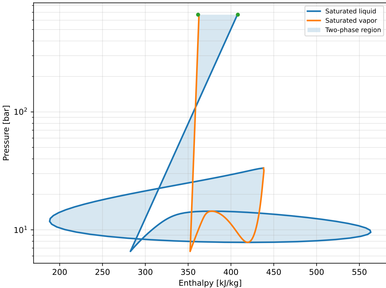
Pure-fluid P-h Saturation Dome
