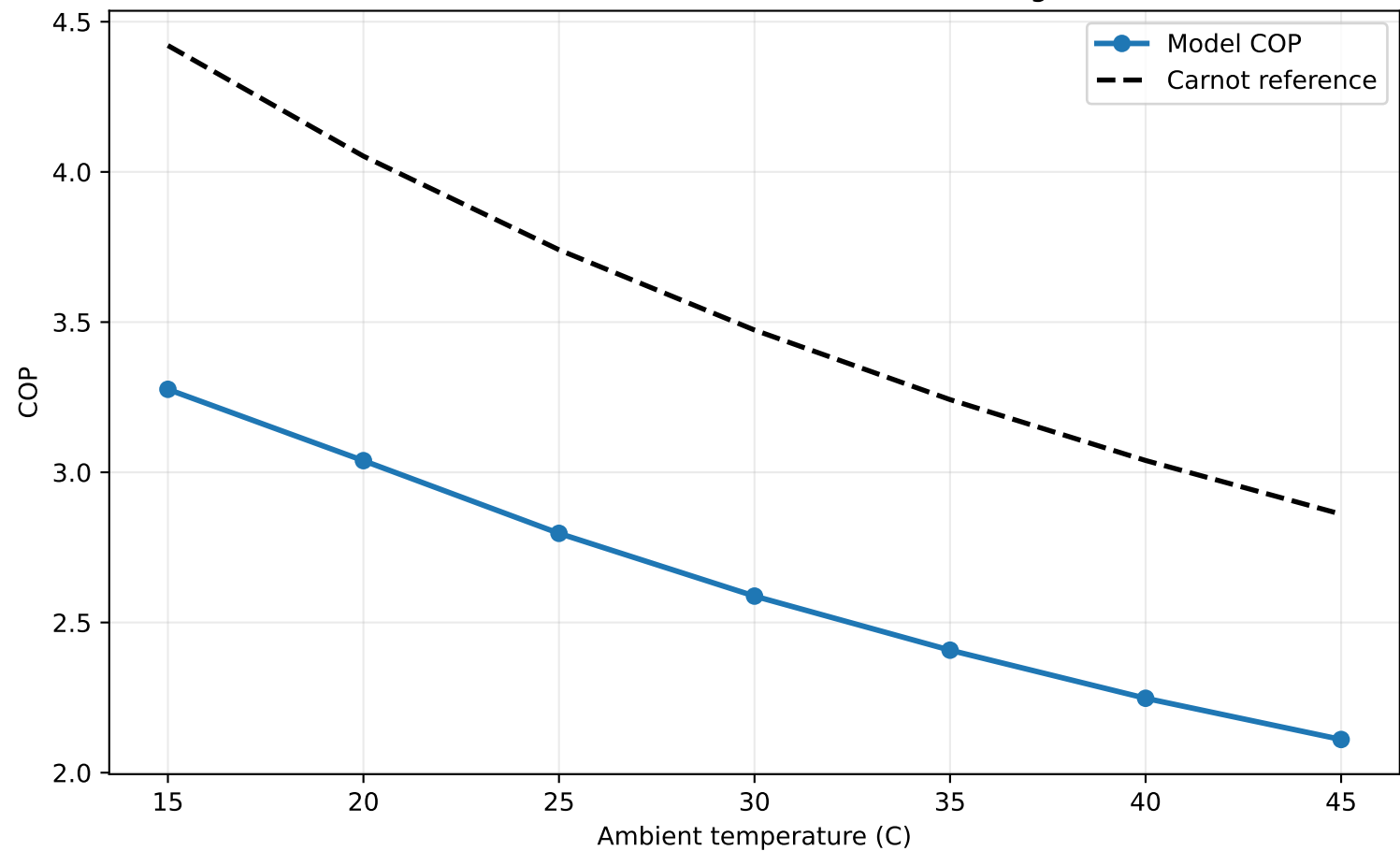
R134a: PLR COP vs Ambient (Cold Storage)
