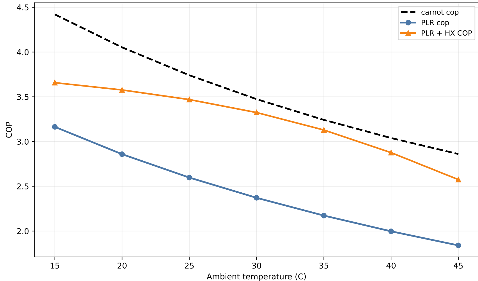
R1234ze(E): COP overlay vs previous Carnot/COP
