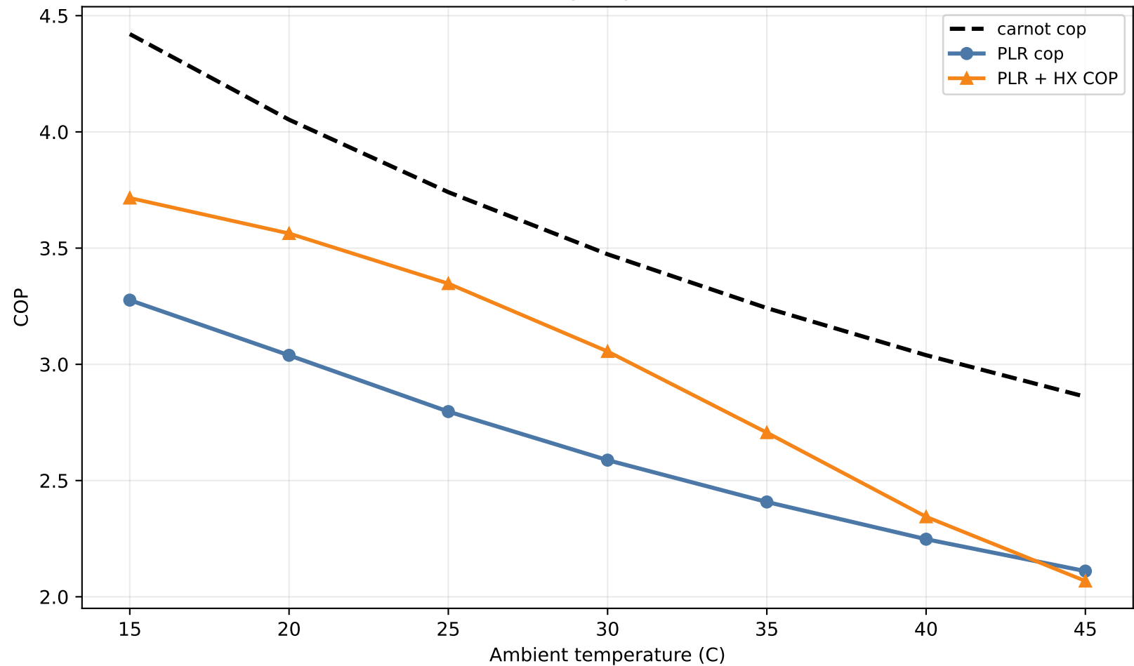
R134a: COP overlay vs previous Carnot/COP
