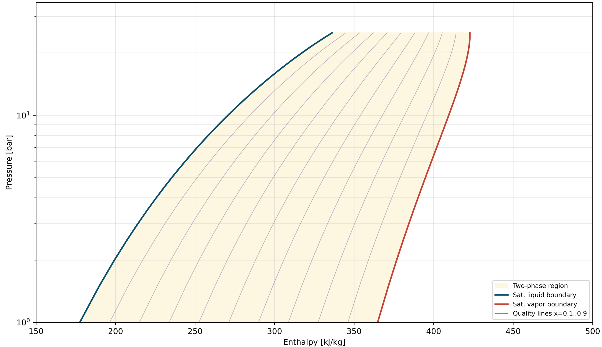
R515B P-h Diagram (Pseudo-pure Honeywell-style composite)
