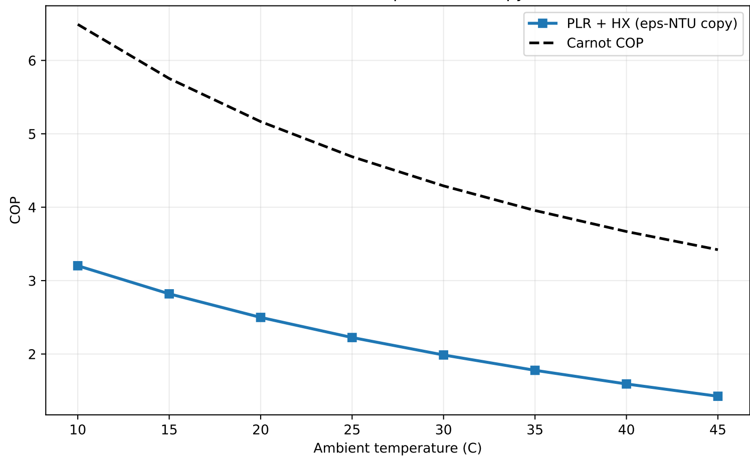
R1234ze(E): Non-IDAES Epsilon-NTU Copy vs Carnot
