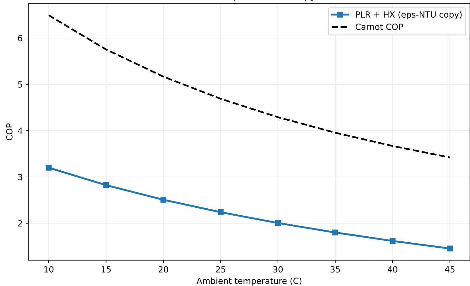
R134a: Non-IDAES Epsilon-NTU Copy vs Carnot
