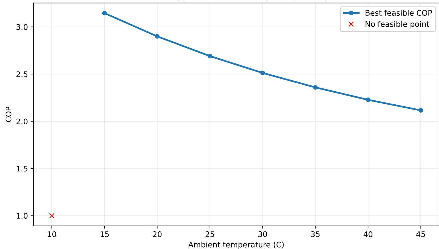
COP vs Ambient (approach=15 C, evap temp sweep -55..-20 C)
