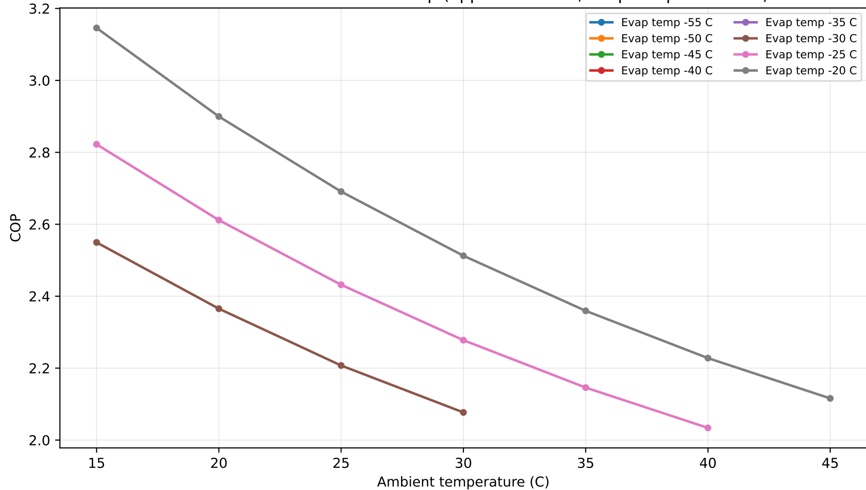
COP vs Ambient from fresh sweep (approach=15 C, evap temp -55..-20 C)
