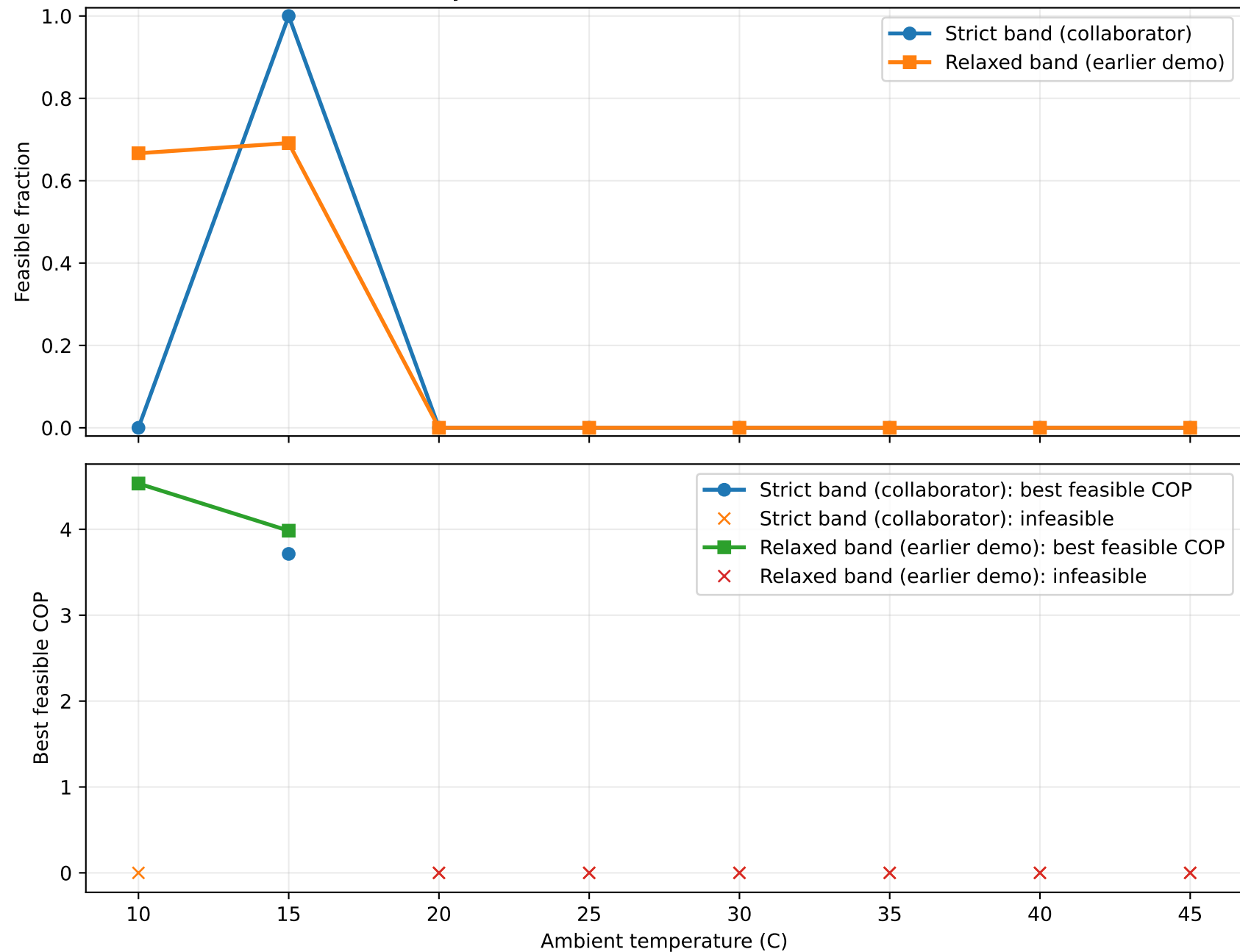
Overlay 1: Strict vs Earlier Relaxed Band (R134a)
