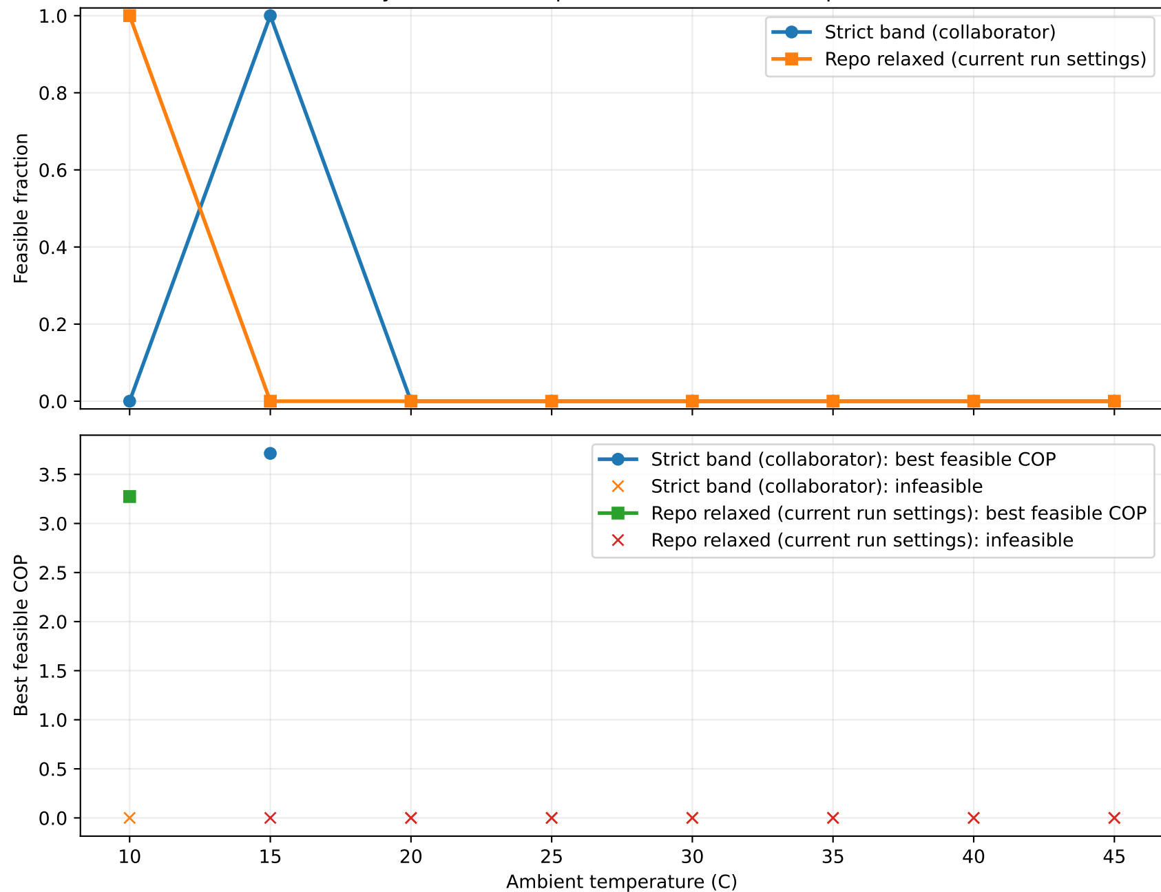
Overlay 2: Strict vs Repo-Current Relaxed Setup (R134a)
